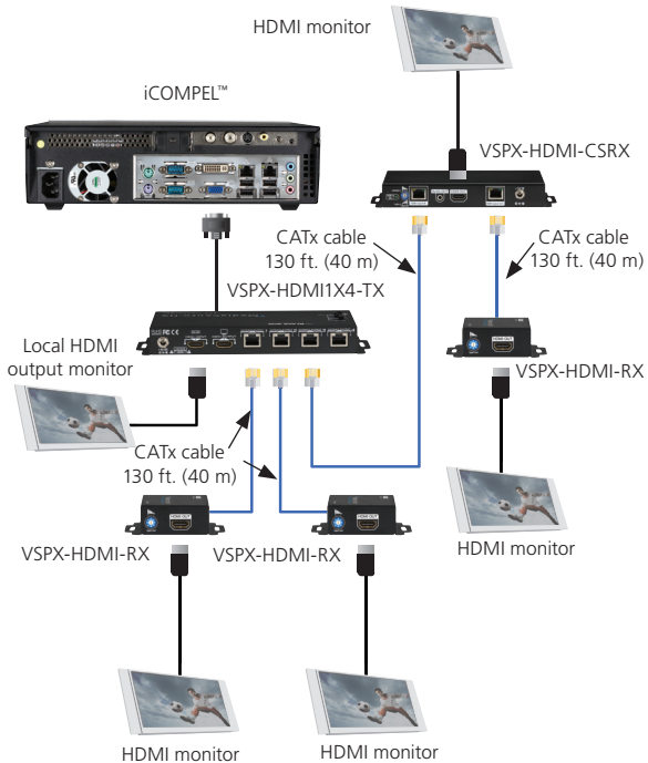
Figure 2-10. Connection diagram #3.
